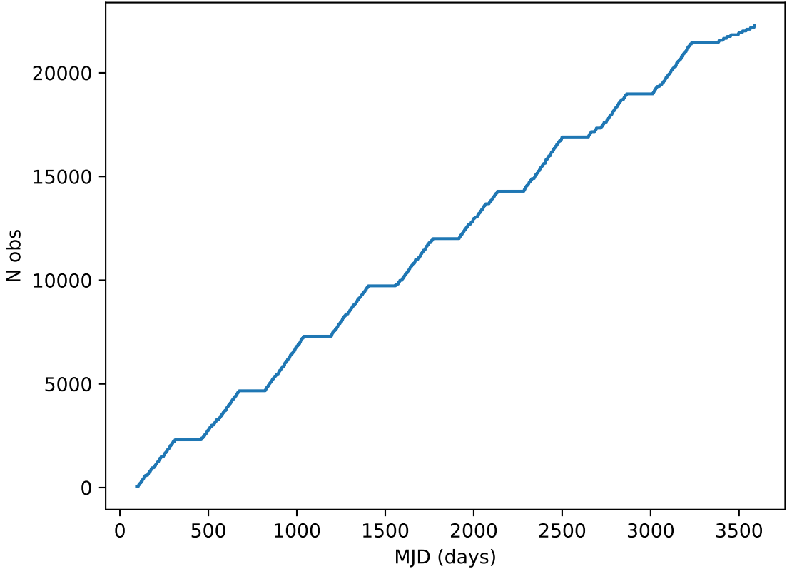
extra_ss_neo5_v3.4_10yrs all bands: DD:ECDFS Cumulative NVisits
