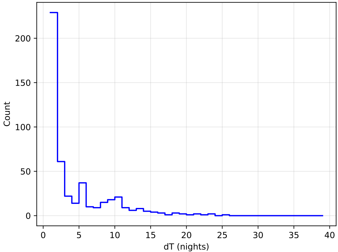
extra_ss_neo5_v3.4_10yrs all bands: DD: COSMOS Delta Nights Histogram
