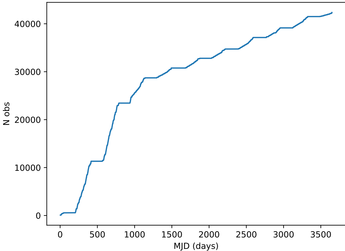
extra_ss_neo5_v3.4_10yrs all bands: DD:COSMOS Cumulative NVisits
