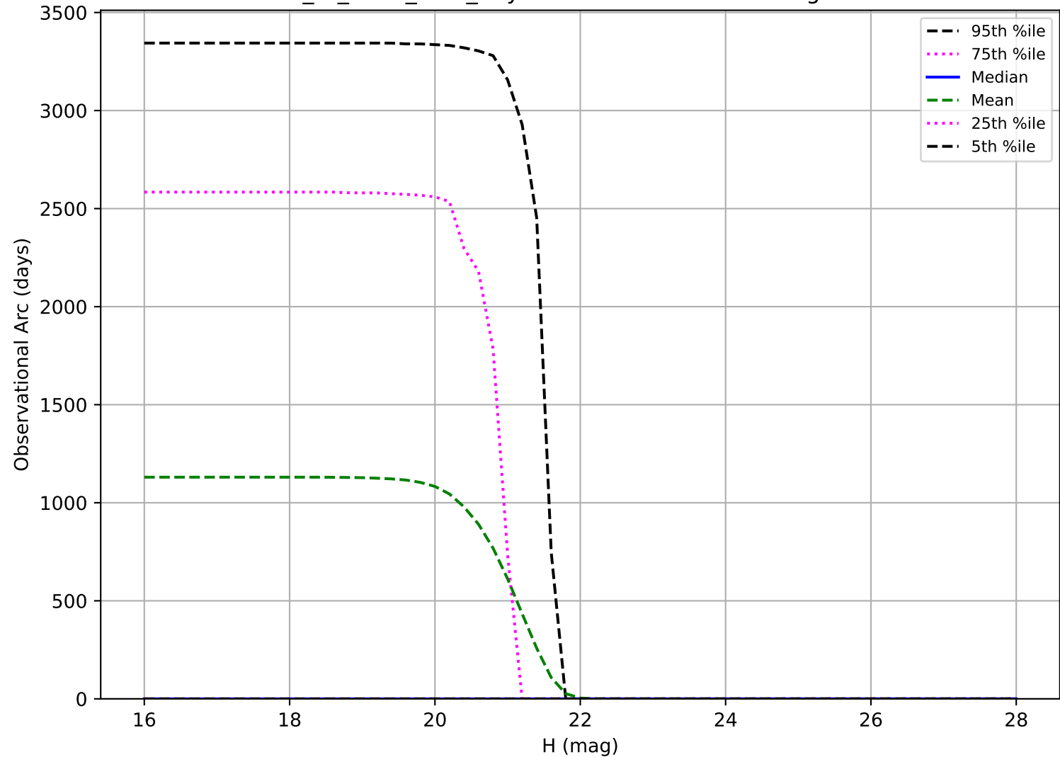
extra_ss_neo4_v3.4_10yrs: Observational Arc Length Vatira
