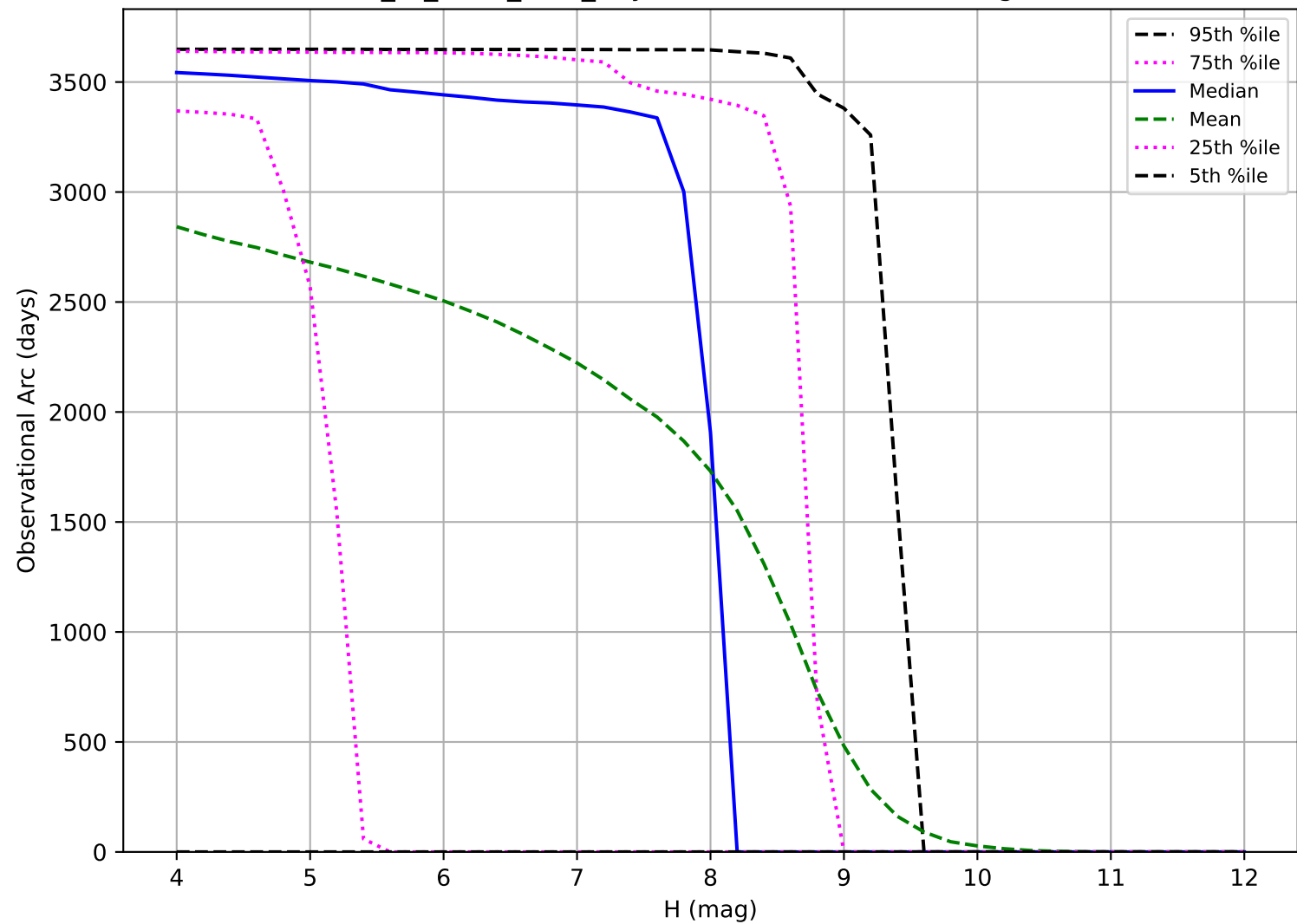
extra_ss_neo4_v3.4_10yrs: Observational Arc Length TNO
