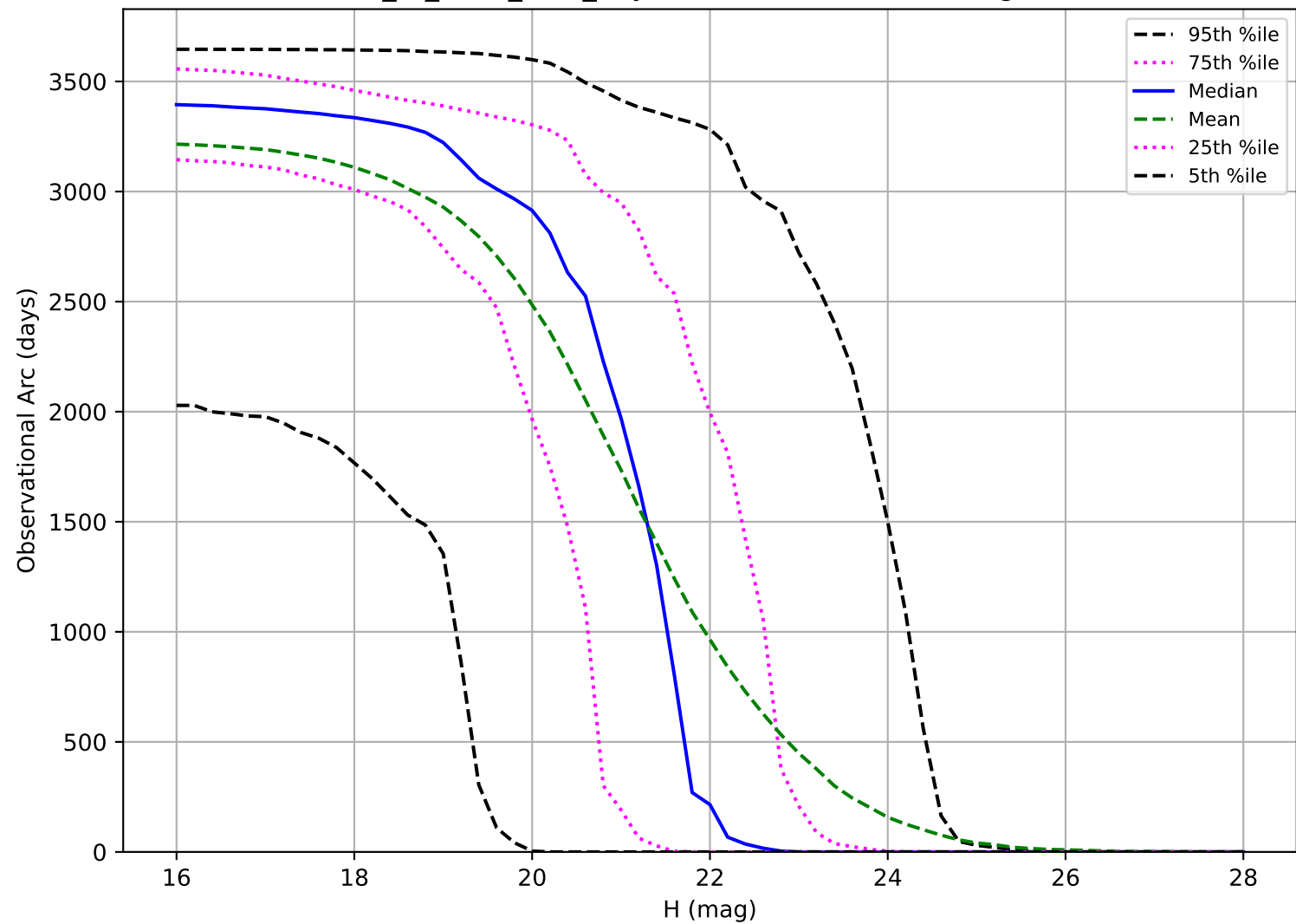
extra_ss_neo4_v3.4_10yrs: Observational Arc Length PHA
