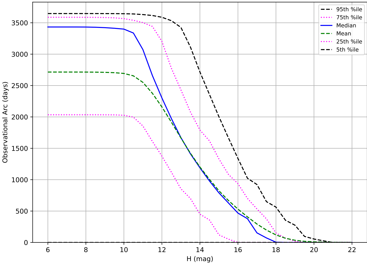
extra_ss_neo4_v3.4_10yrs: Observational Arc Length OCC_r5
