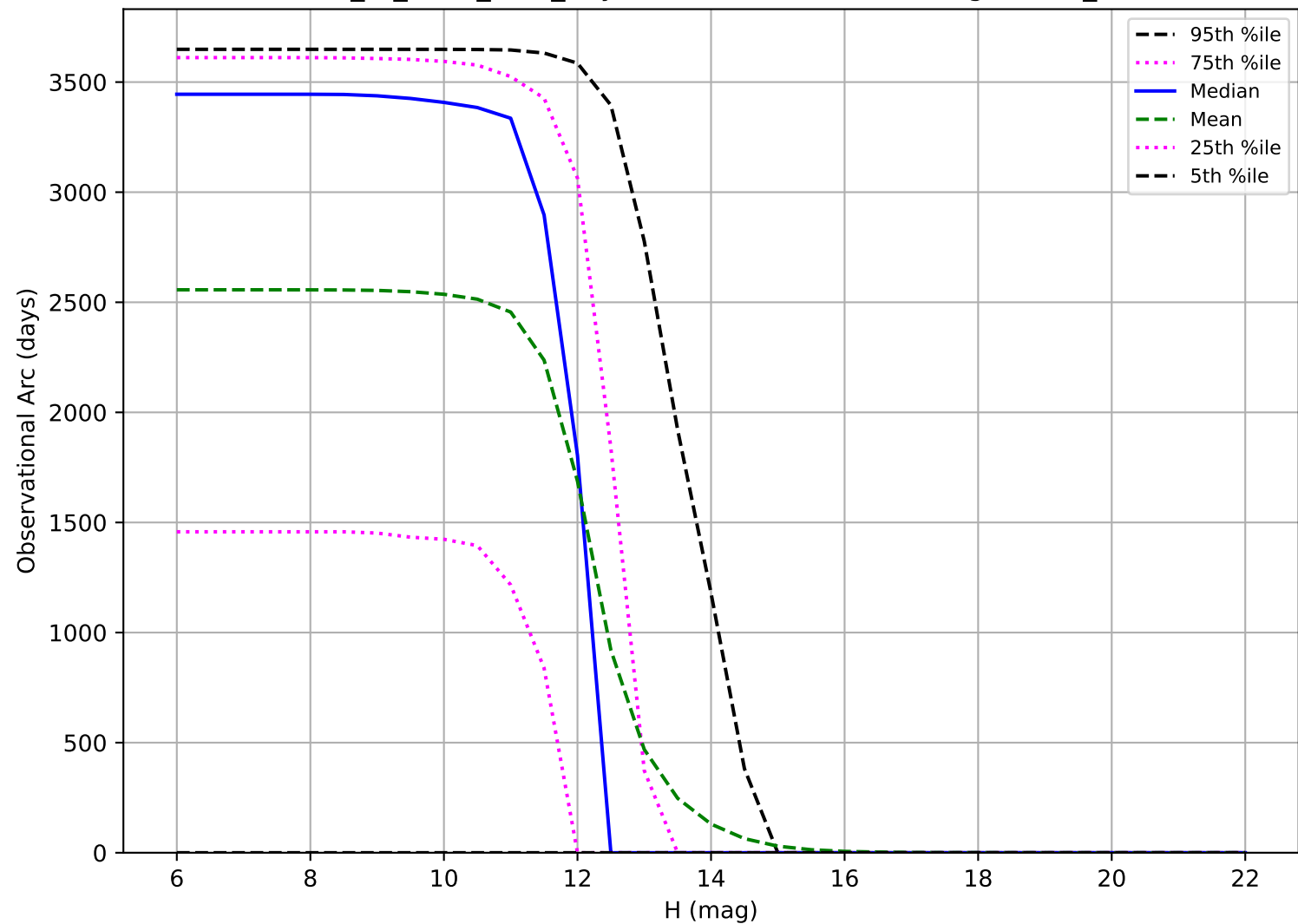
extra_ss_neo4_v3.4_10yrs: Observational Arc Length OCC_r20
