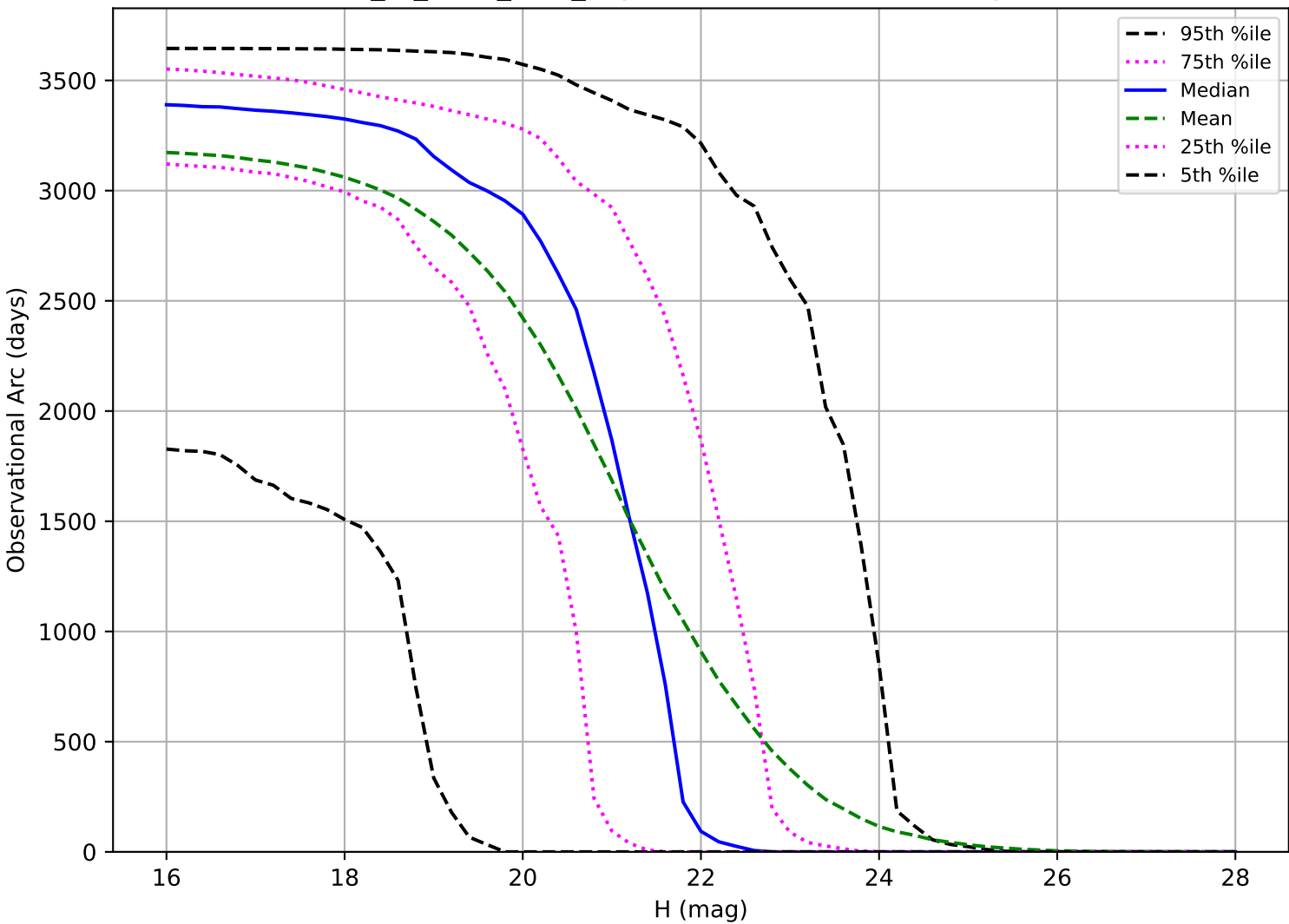
extra_ss_neo4_v3.4_10yrs: Observational Arc Length NEO
