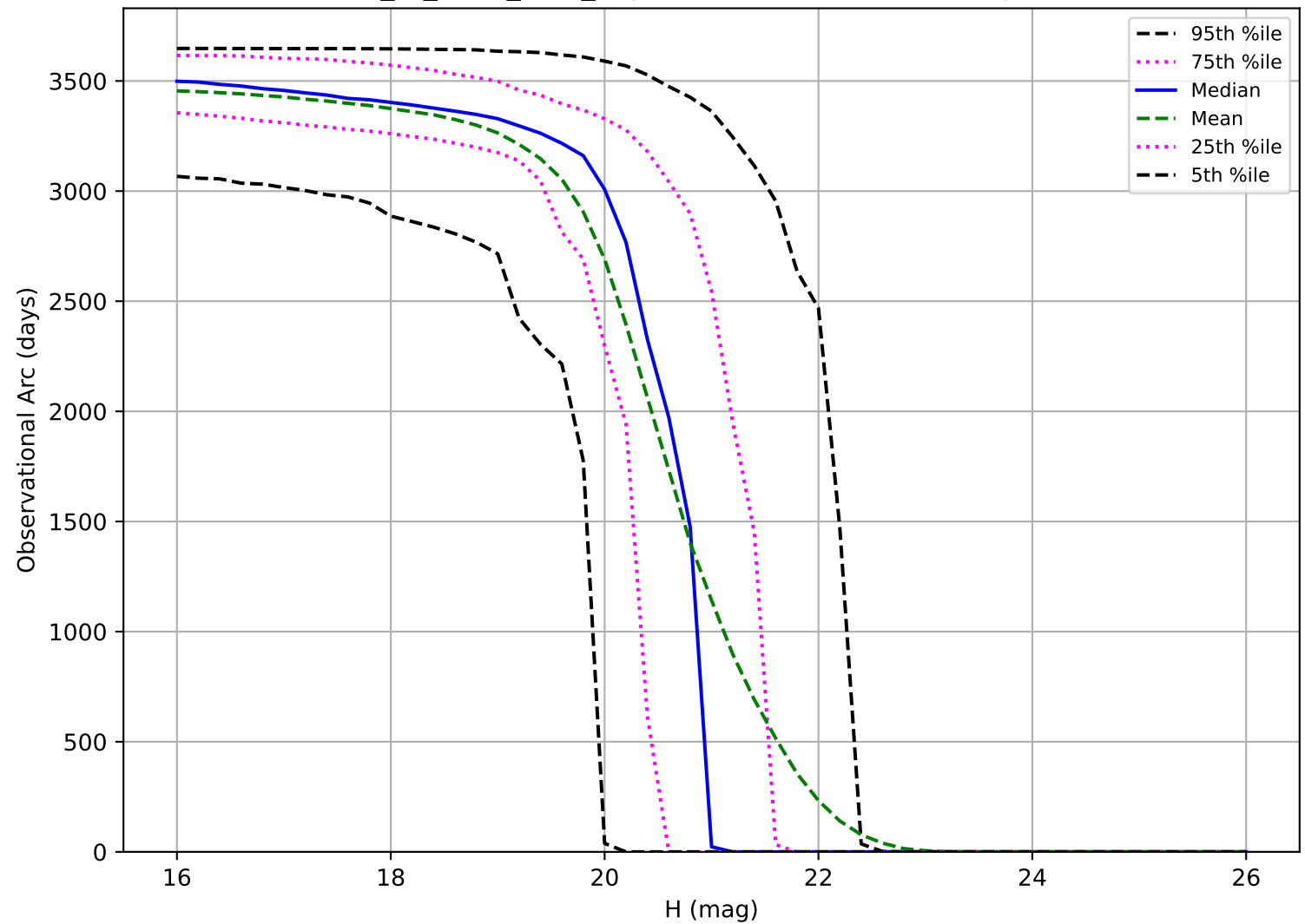
extra_ss_neo4_v3.4_10yrs: Observational Arc Length MBA
