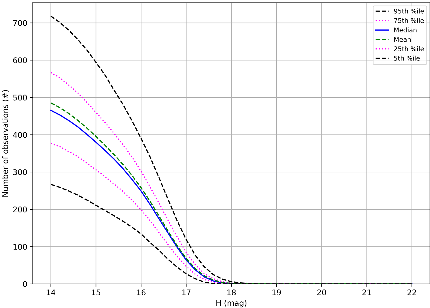
extra_ss_neo4_v3.4_10yrs: Number of observations Trojan
