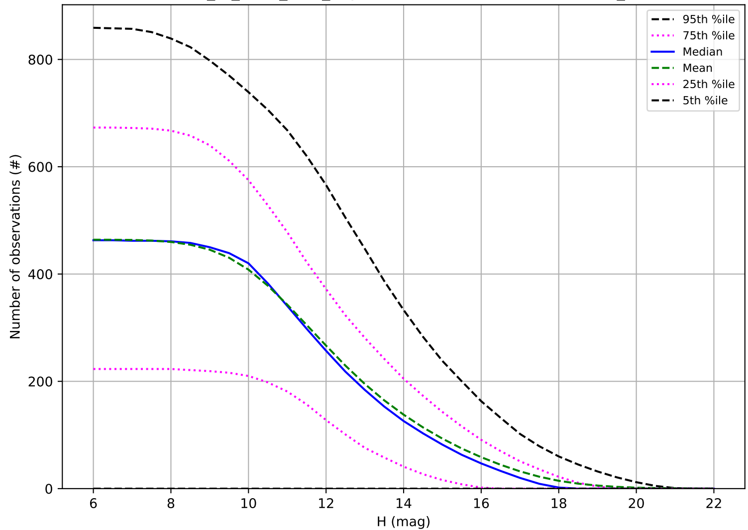
extra_ss_neo4_v3.4_10yrs: Number of observations OCC_r5
