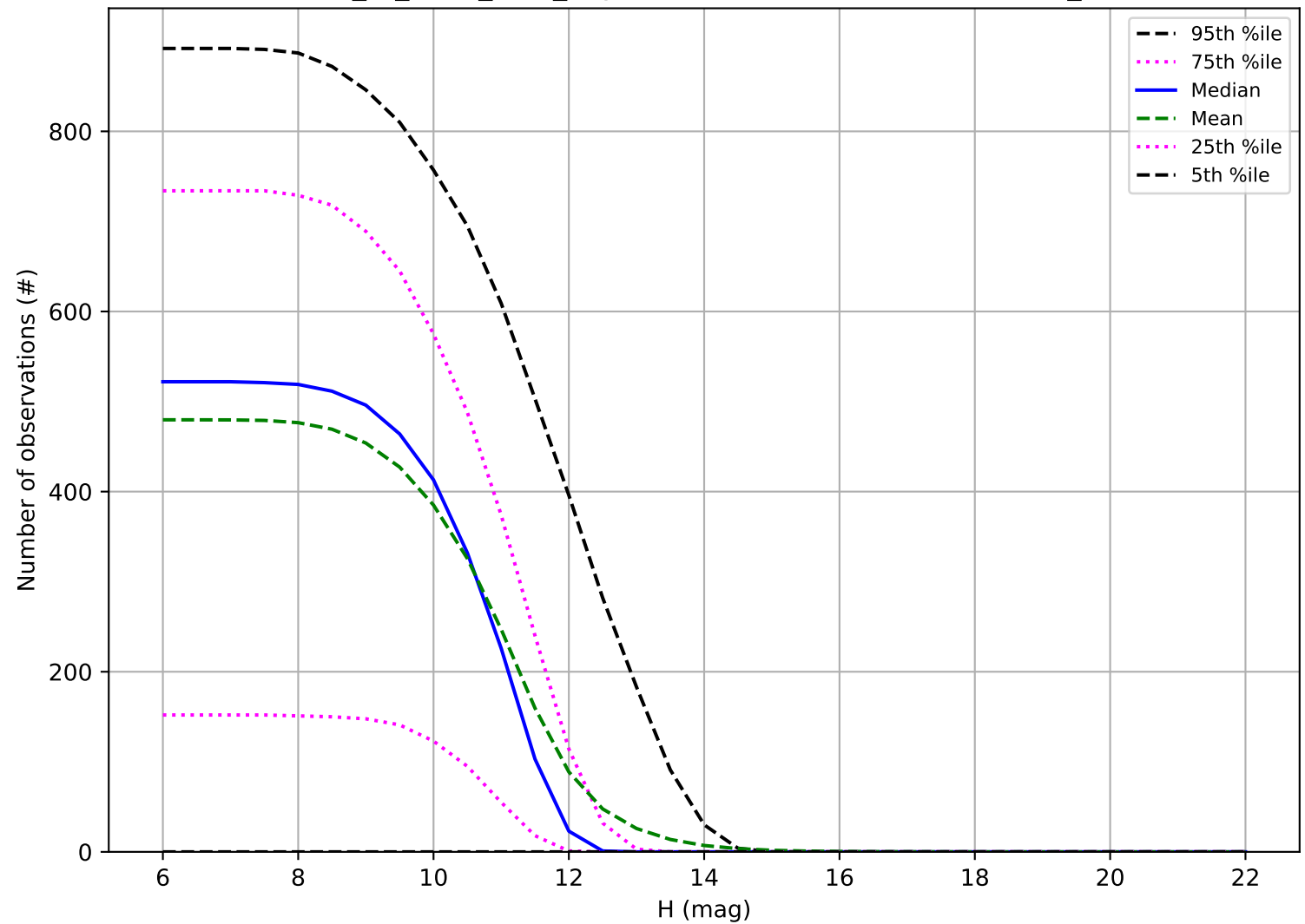
extra_ss_neo4_v3.4_10yrs: Number of observations OCC_r20
