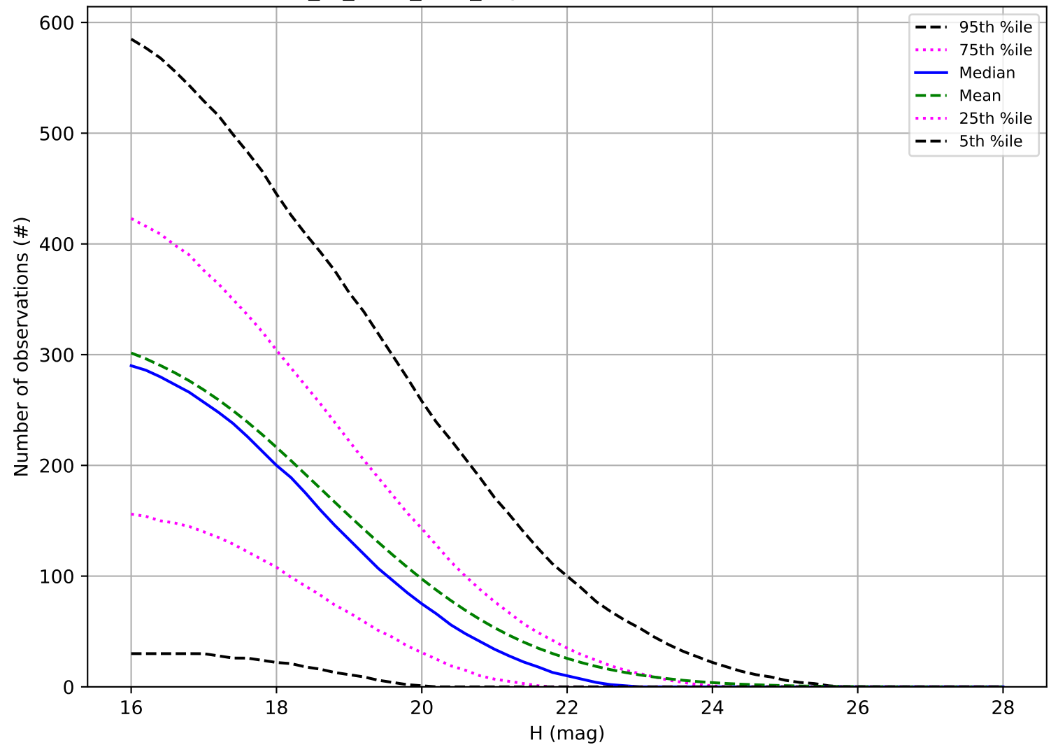
extra_ss_neo4_v3.4_10yrs: Number of observations NEO
