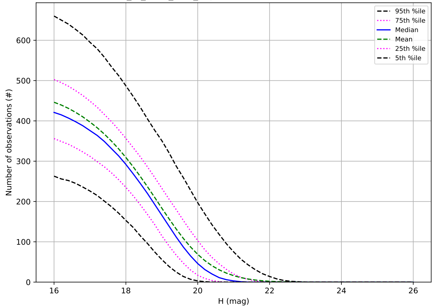
extra_ss_neo4_v3.4_10yrs: Number of observations MBA
