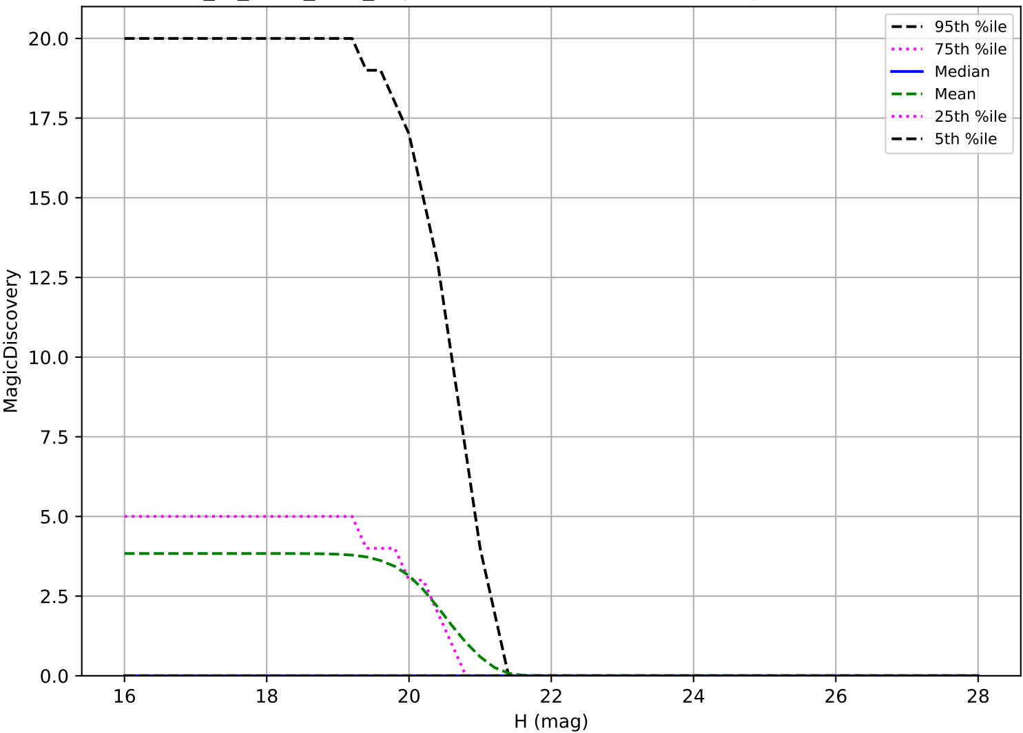
extra_ss_neo4_v3.4_10yrs: Vatira 6 detections in 60 nights detection loss
