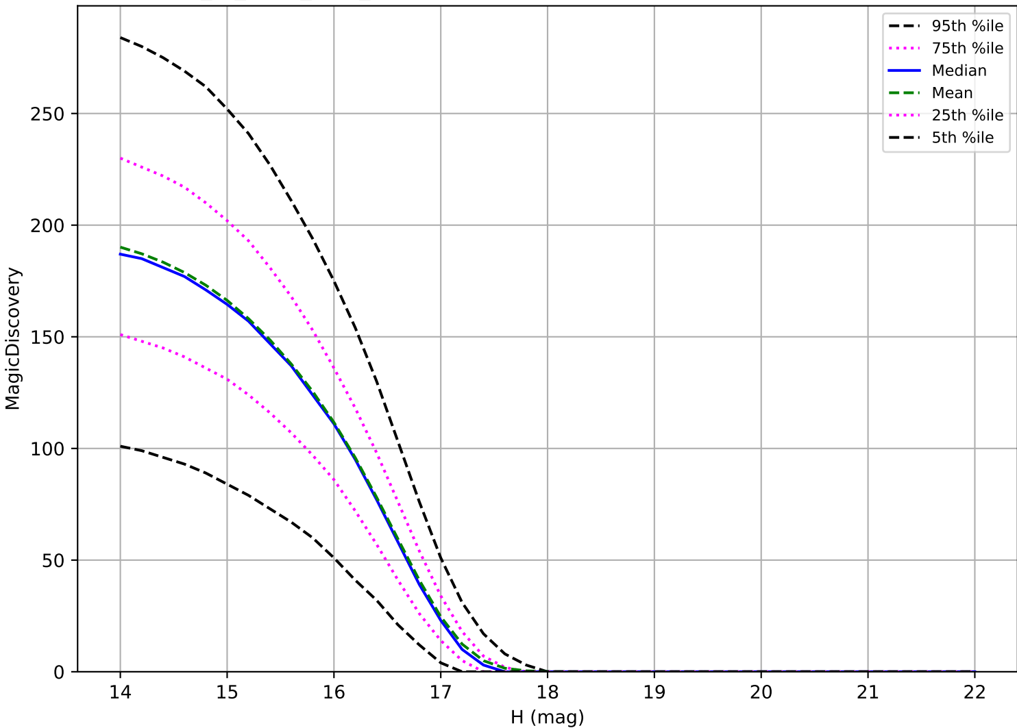
extra_ss_neo4_v3.4_10yrs: Trojan 6 detections in 60 nights detection loss
