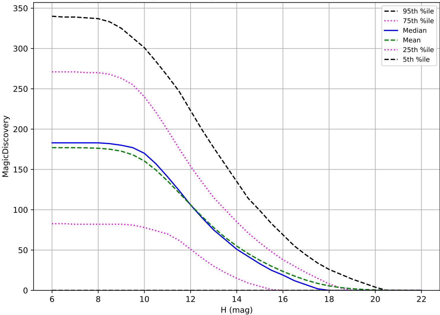
extra_ss_neo4_v3.4_10yrs: OCC_r5 6 detections in 60 nights detection loss
