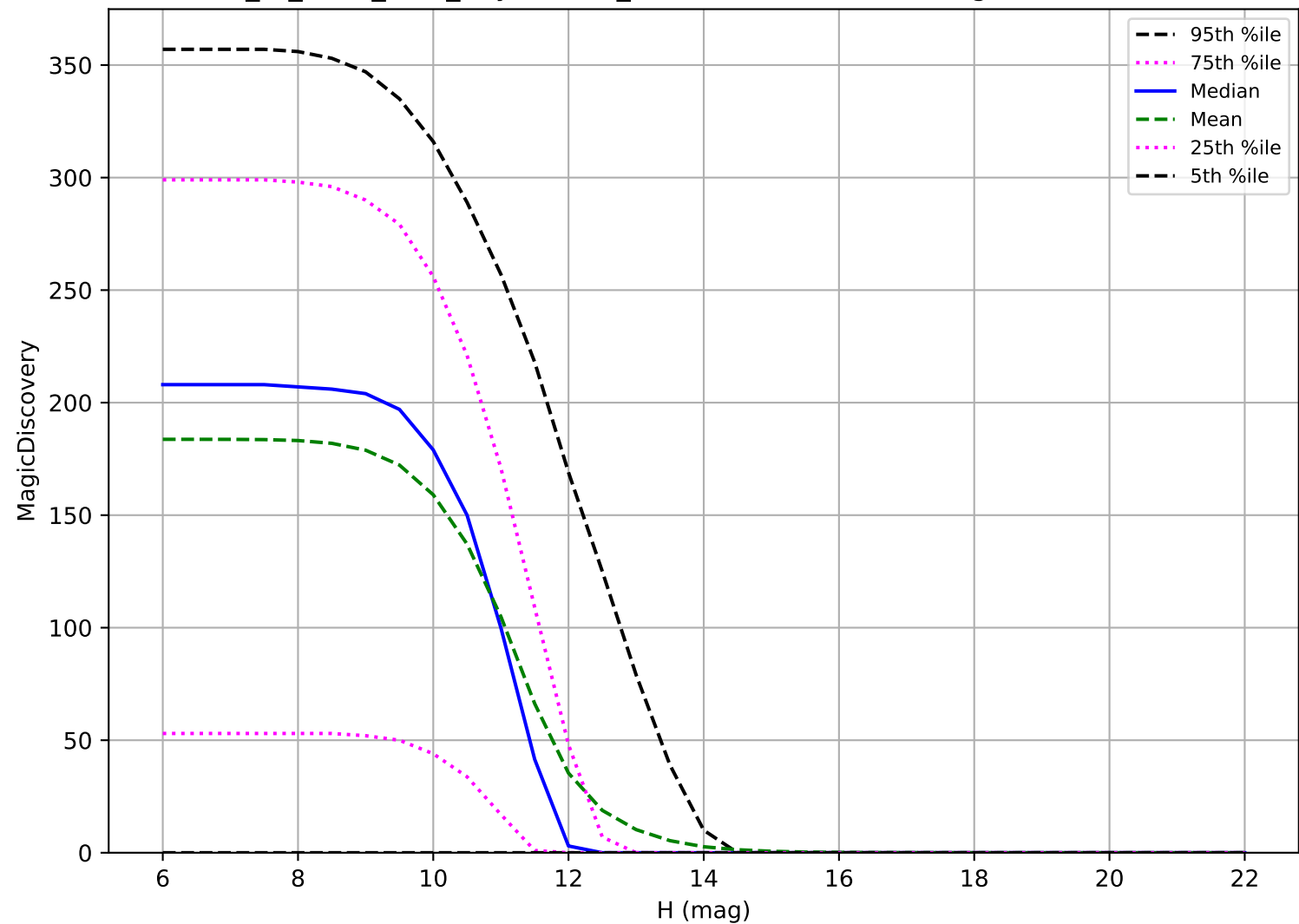
extra_ss_neo4_v3.4_10yrs: OCC_r20 6 detections in 60 nights detection loss
