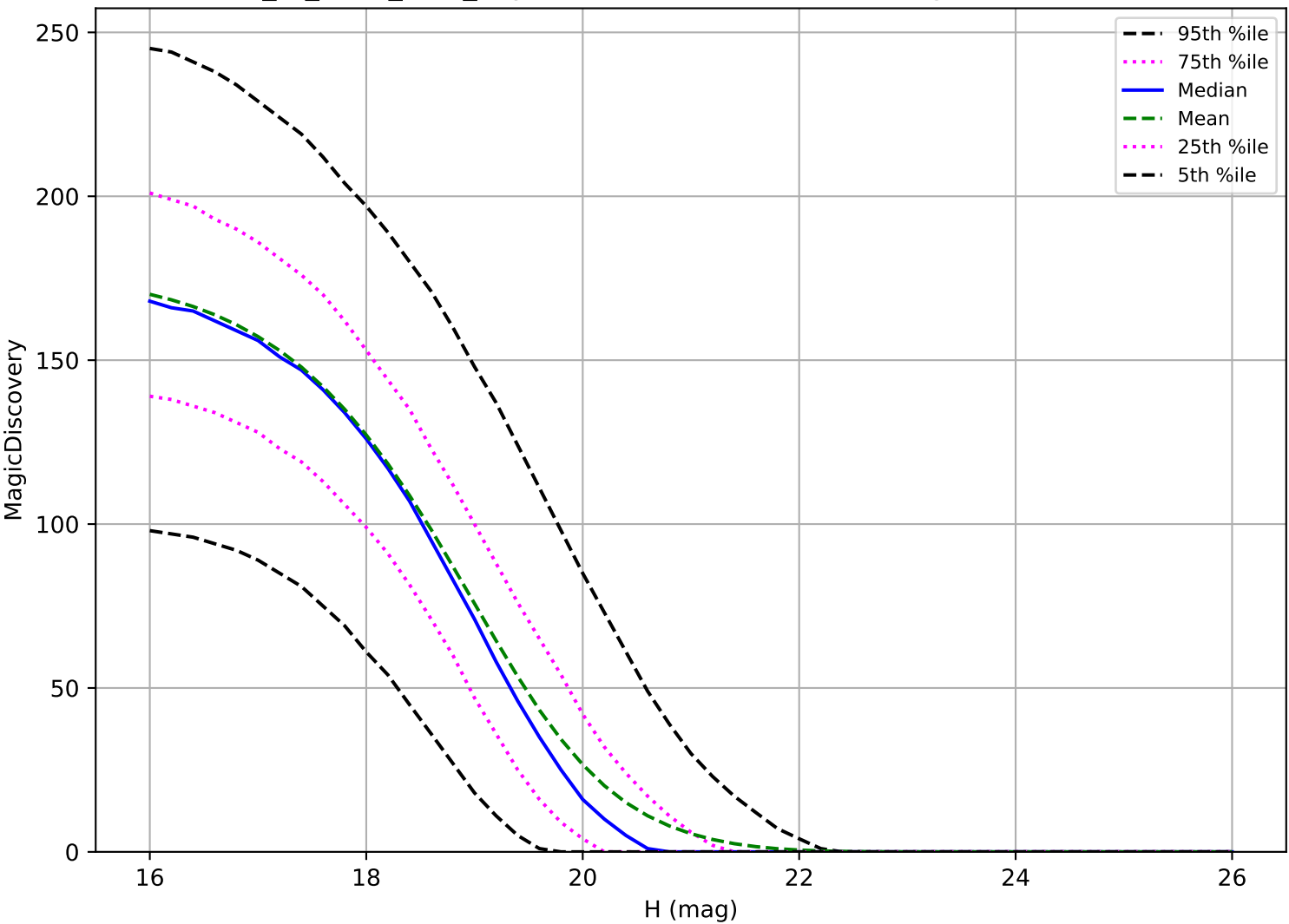
extra_ss_neo4_v3.4_10yrs: MBA 6 detections in 60 nights detection loss
