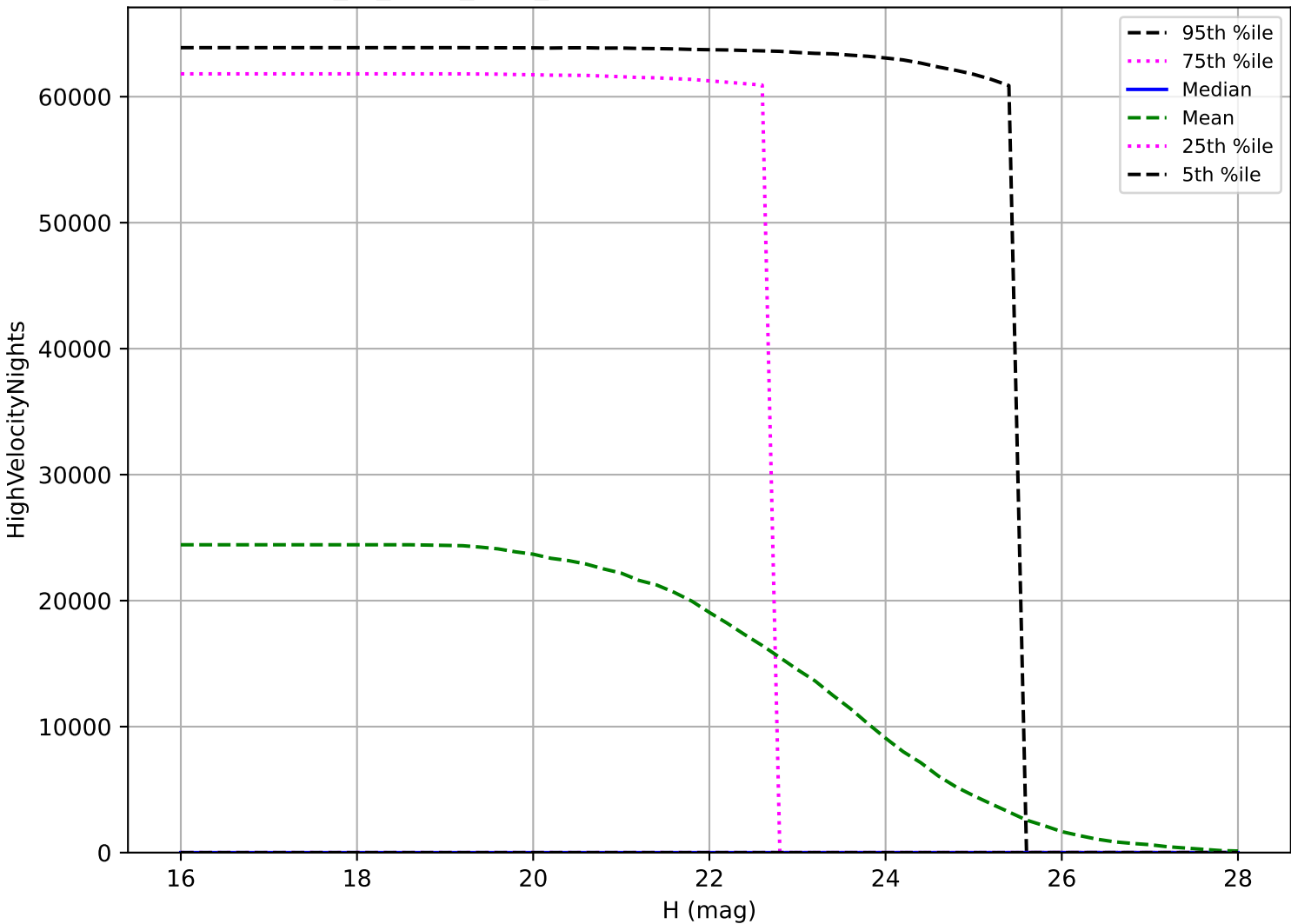
extra_ss_neo4_v3.4_10yrs: PHA High velocity pair detection loss
