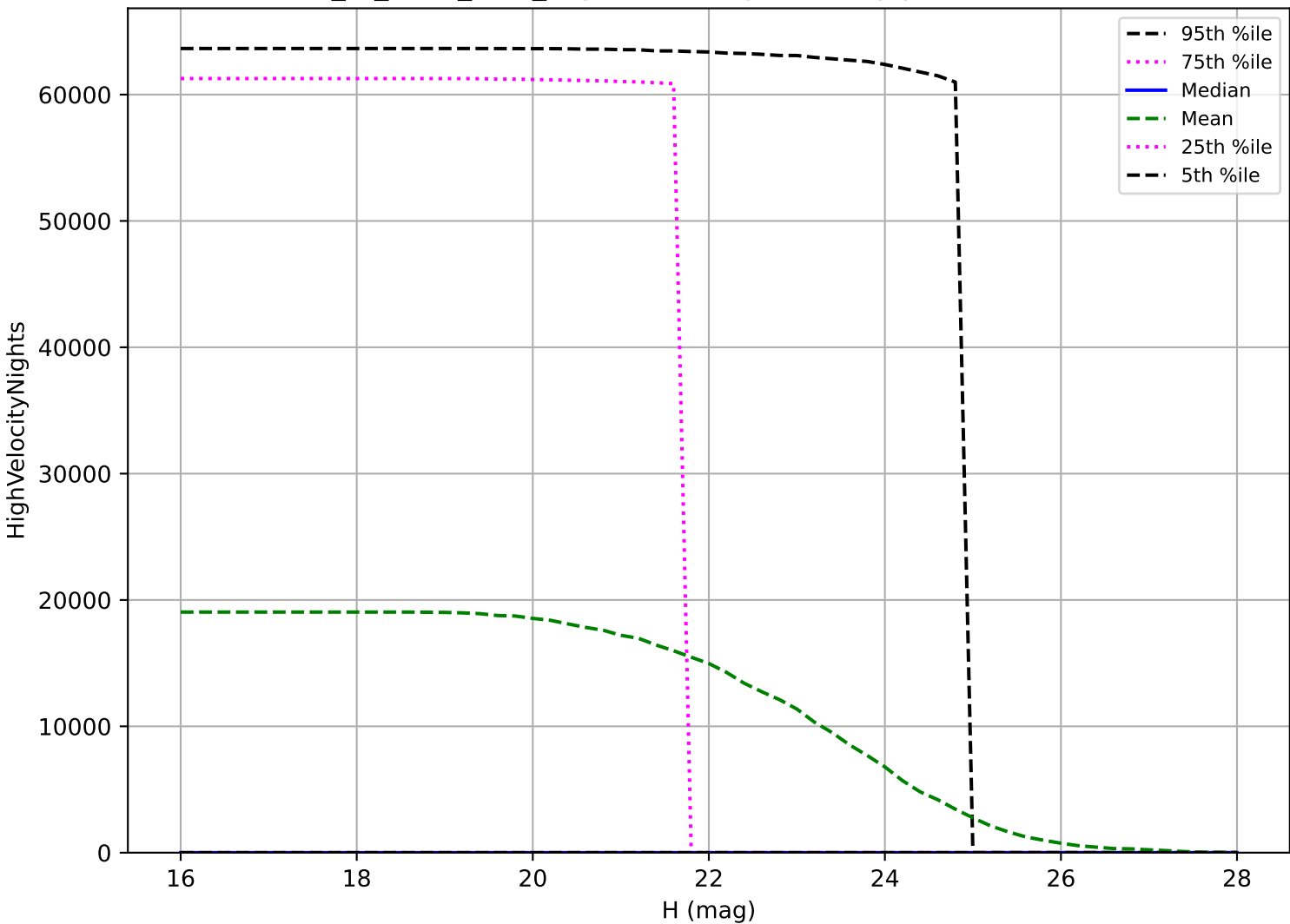
extra_ss_neo4_v3.4_10yrs: NEO High velocity pair detection loss
