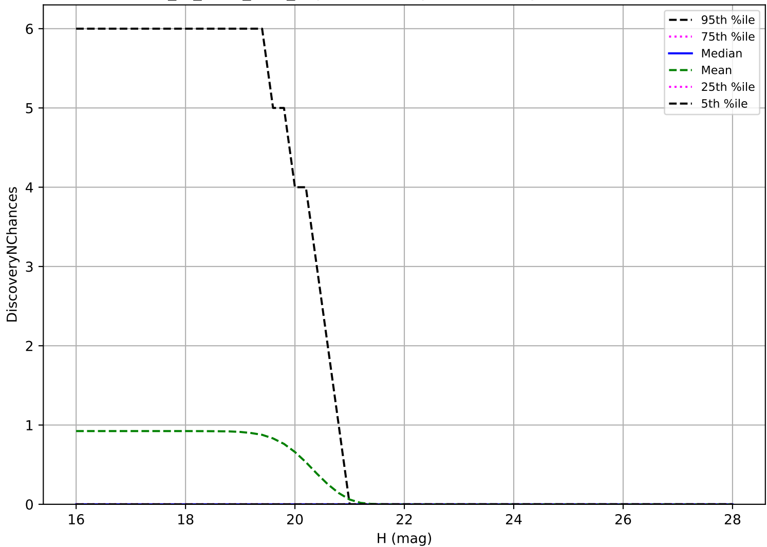
extra_ss_neo4_v3.4_10yrs: Vatira 3 pairs in 15 nights detection loss
