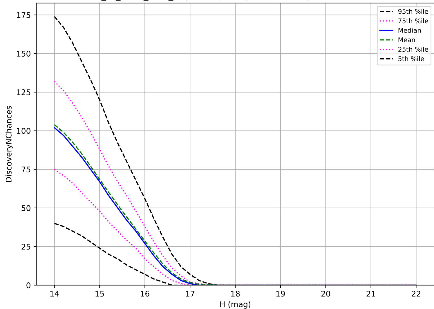
extra_ss_neo4_v3.4_10yrs: Trojan 3 pairs in 15 nights detection loss
