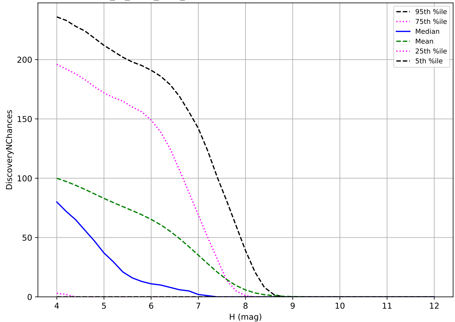
extra_ss_neo4_v3.4_10yrs: TNO 3 pairs in 15 nights detection loss
