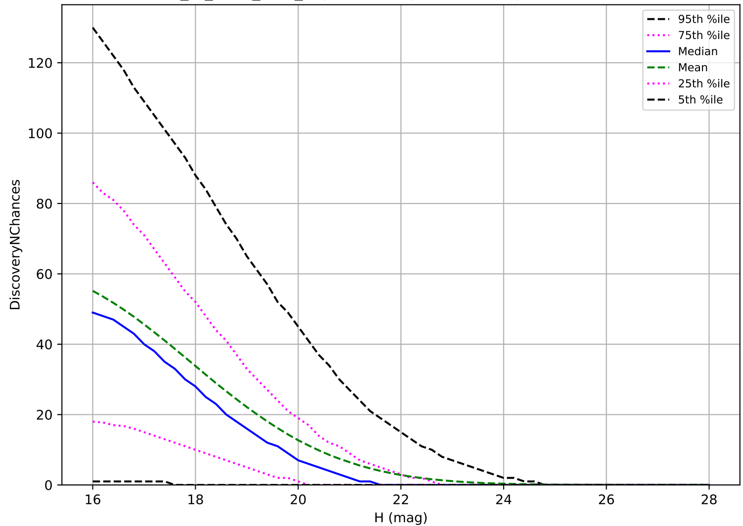
extra_ss_neo4_v3.4_10yrs: PHA 3 pairs in 15 nights detection loss
