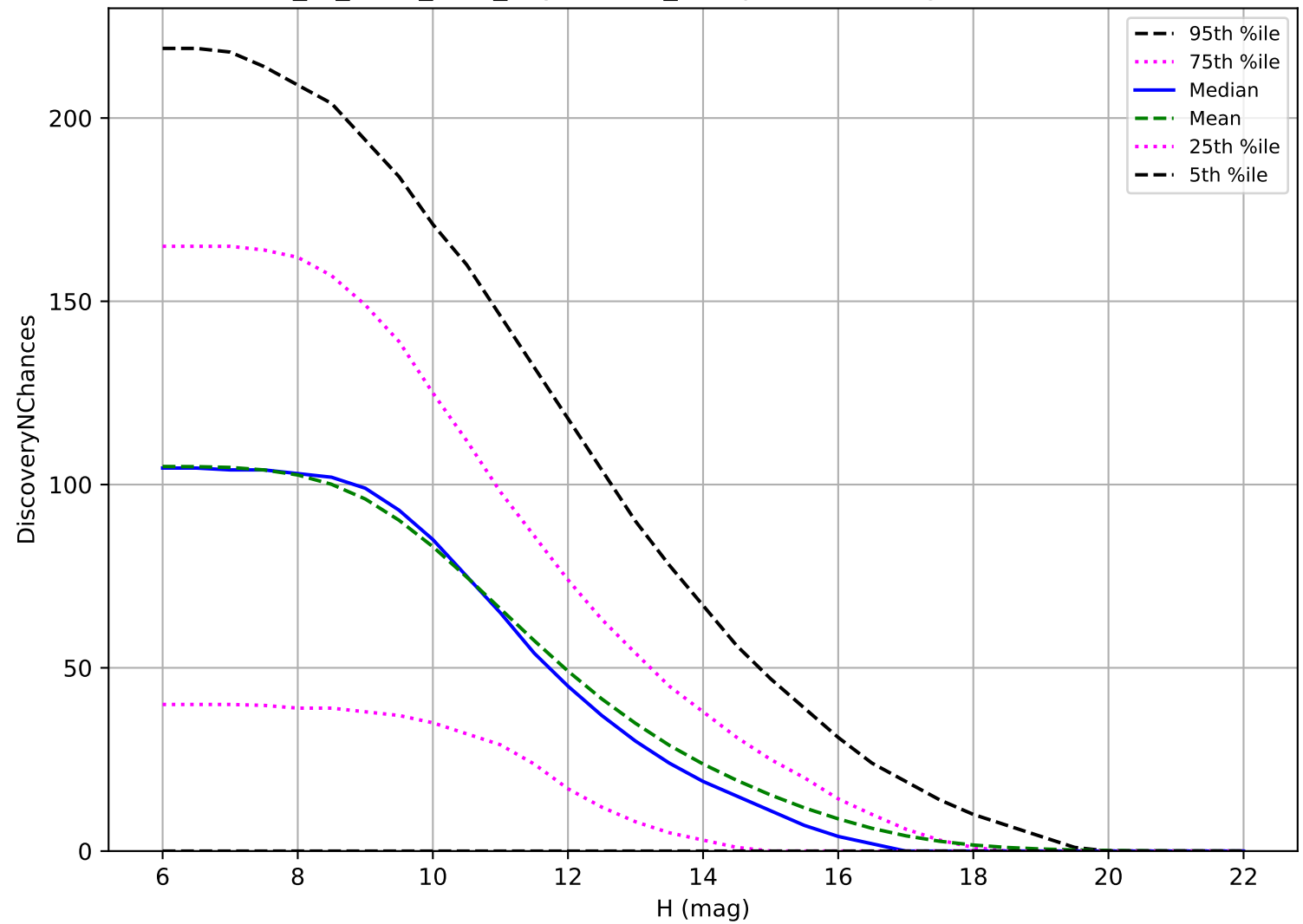
extra_ss_neo4_v3.4_10yrs: OCC_r5 3 pairs in 15 nights detection loss
