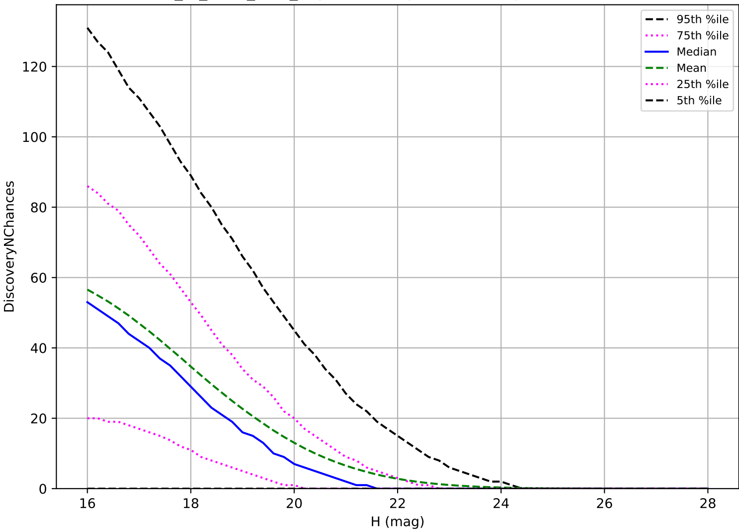
extra_ss_neo4_v3.4_10yrs: NEO 3 pairs in 15 nights detection loss
