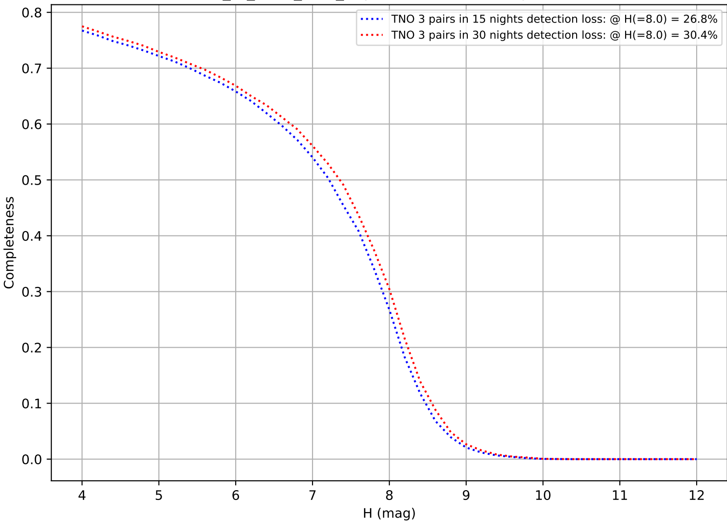
extra_ss_neo4_v3.4_10yrs: DifferentialCompleteness
