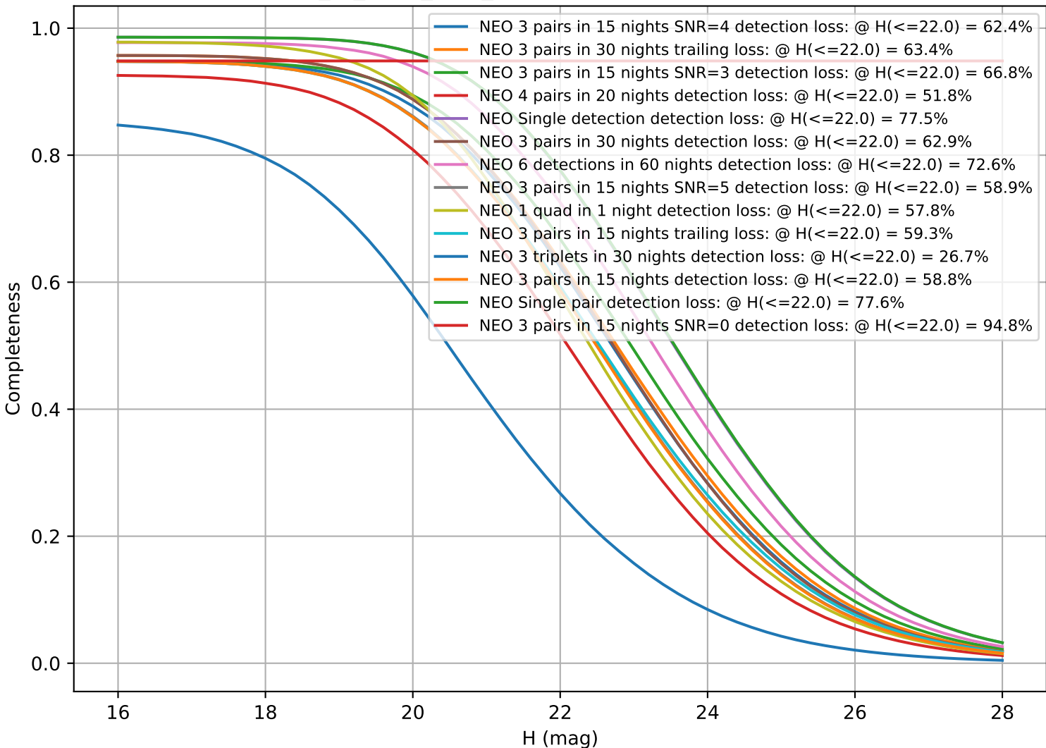
extra_ss_neo4_v3.4_10yrs: CumulativeCompleteness
