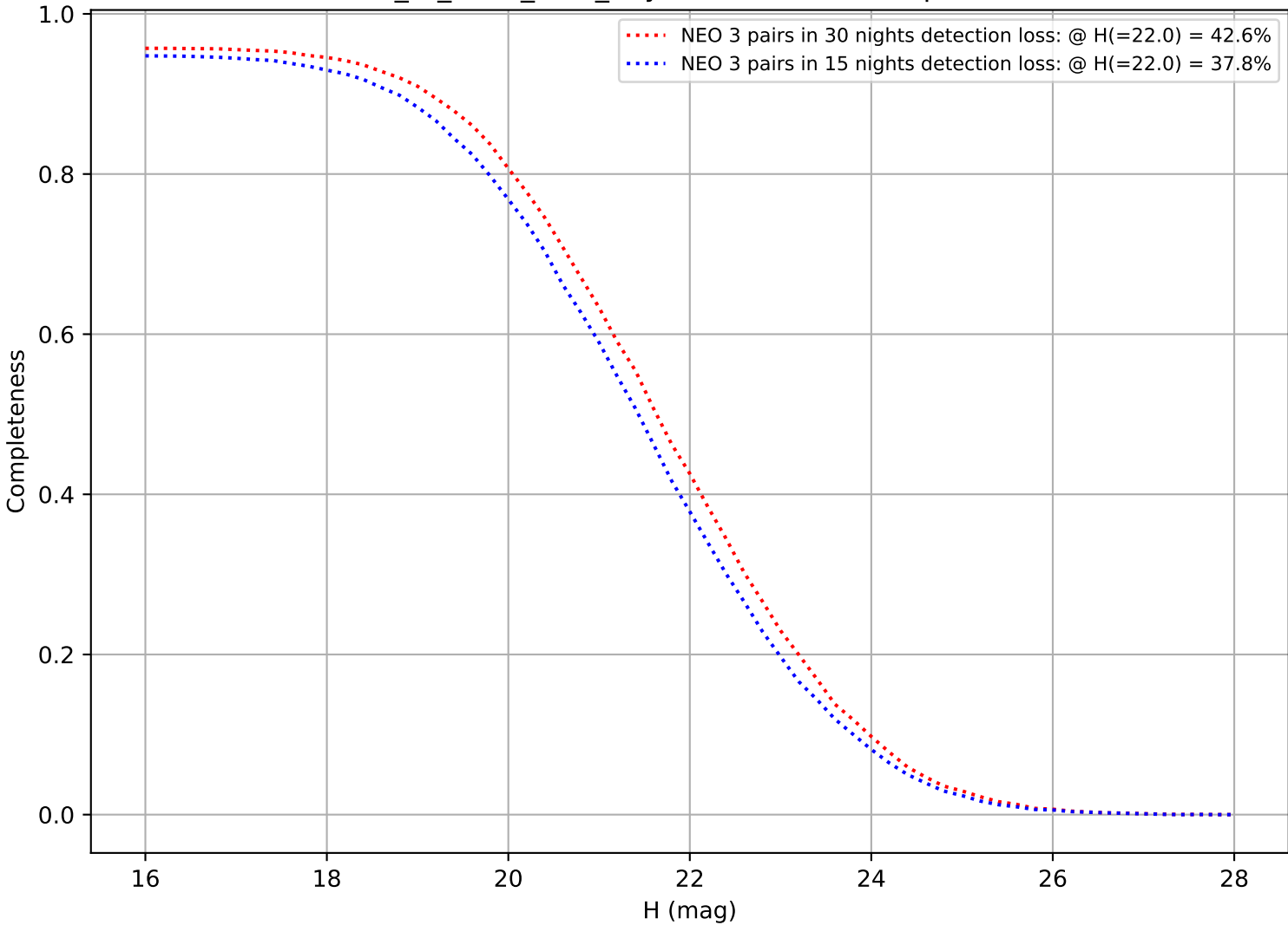
extra_ss_neo4_v3.4_10yrs: DifferentialCompleteness
