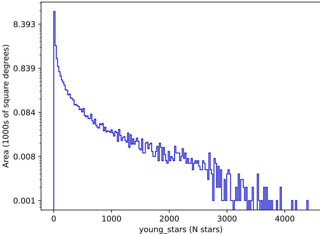
extra_ss_neo4_v3.4_10yrs : young_stars
