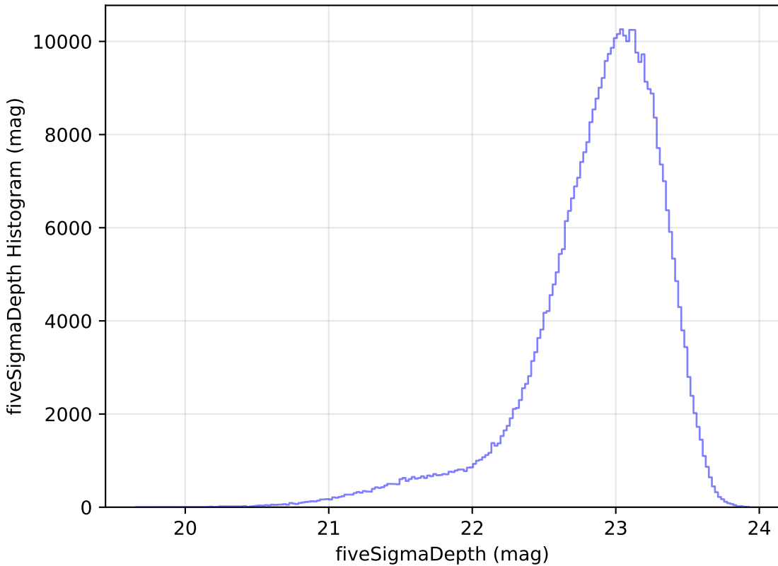
extra_ss_neo4_v3.4_10yrs z: fiveSigmaDepth Histogram
