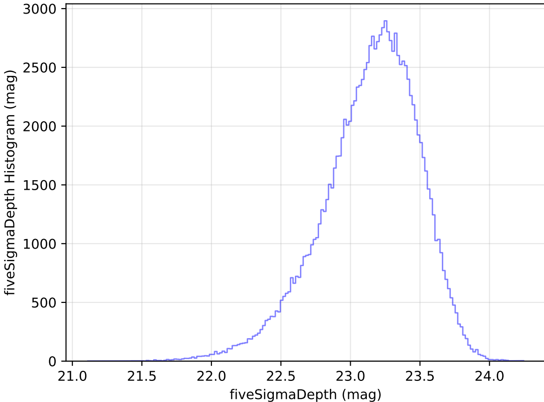
extra_ss_neo4_v3.4_10yrs u: fiveSigmaDepth Histogram
