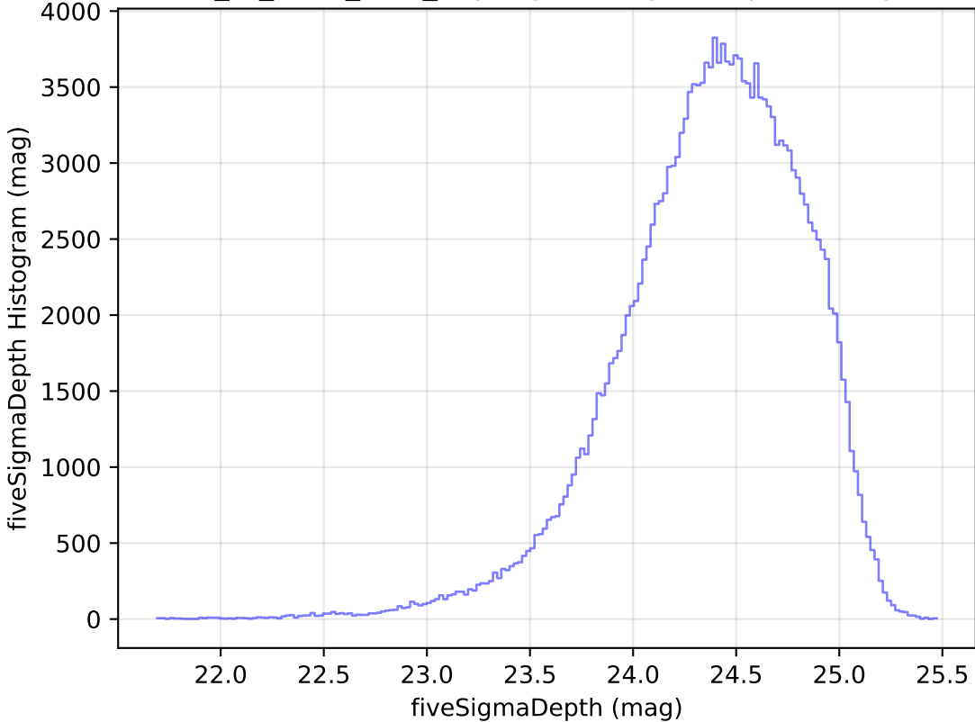
extra_ss_neo4_v3.4_10yrs g: fiveSigmaDepth Histogram
