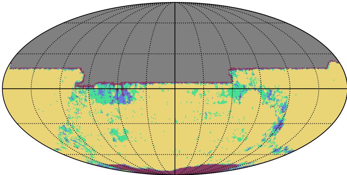
extra_ss_neo4_v3.4_10yrs y band: YearCoverage night
