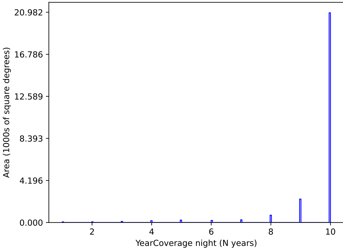
extra_ss_neo4_v3.4_10yrs y band: YearCoverage night
