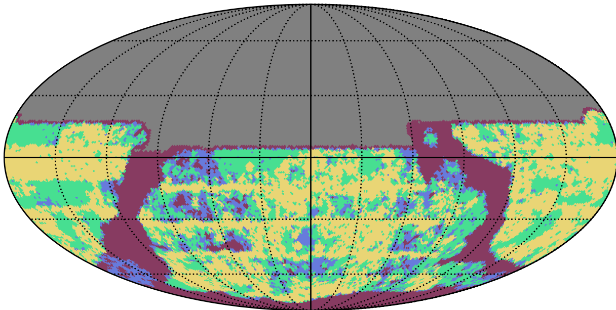
extra_ss_neo4_v3.4_10yrs u band: YearCoverage night
