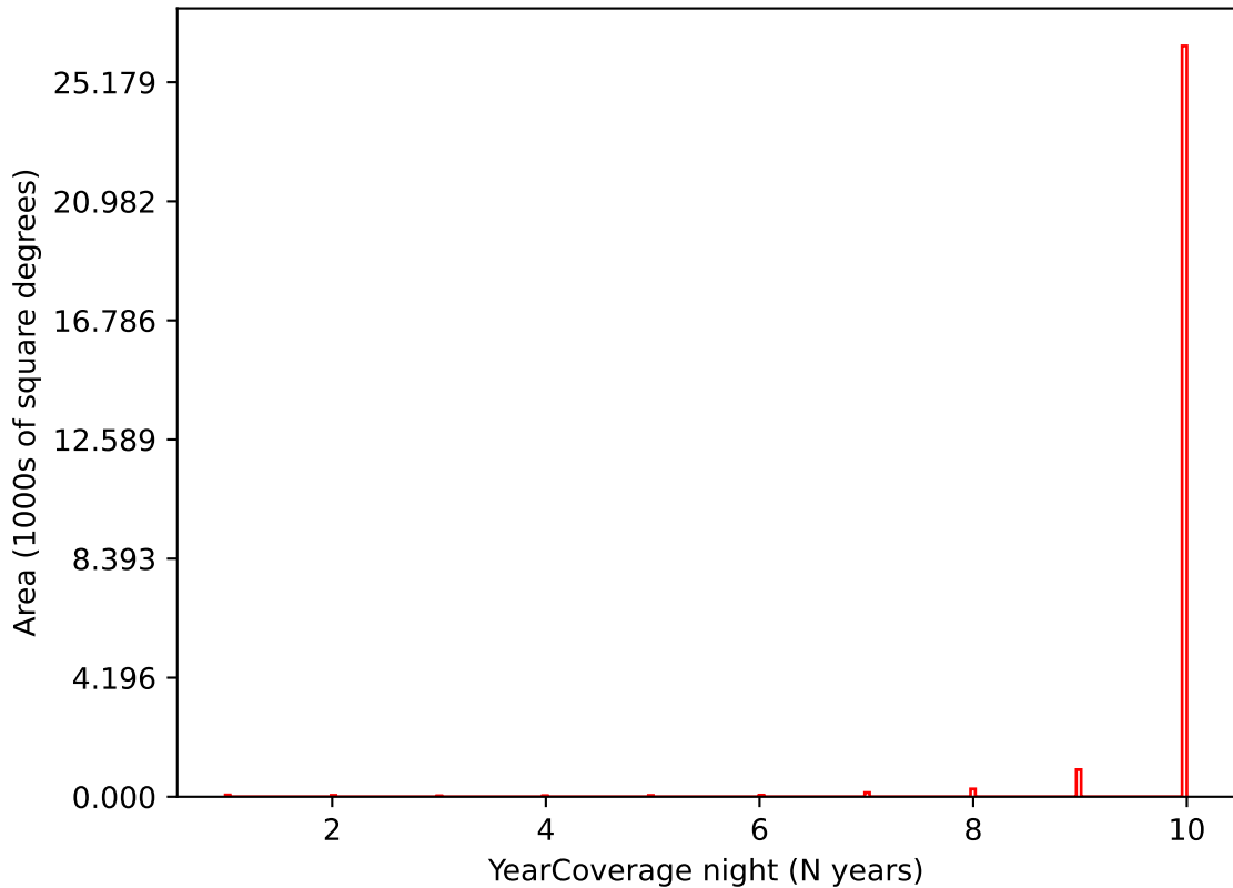
extra_ss_neo4_v3.4_10yrs i band: YearCoverage night
