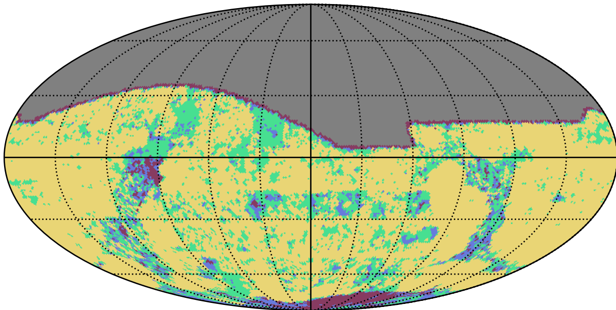
extra_ss_neo4_v3.4_10yrs g band: YearCoverage night
