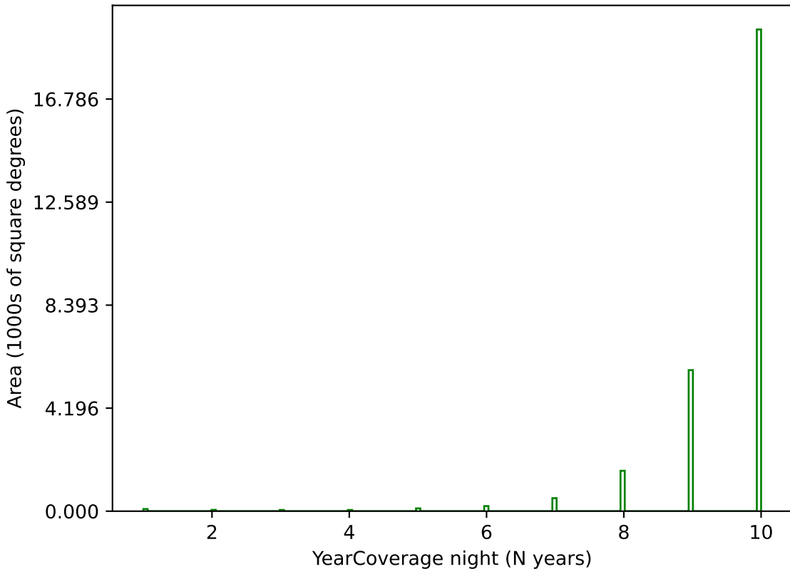
extra_ss_neo4_v3.4_10yrs g band: YearCoverage night
