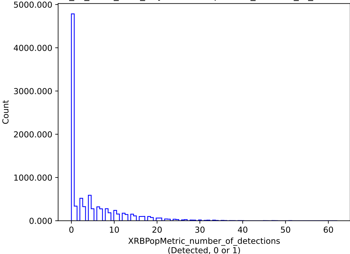
extra_ss_neo4_v3.4_10yrs : XRBPoMetric_number_of_detections
