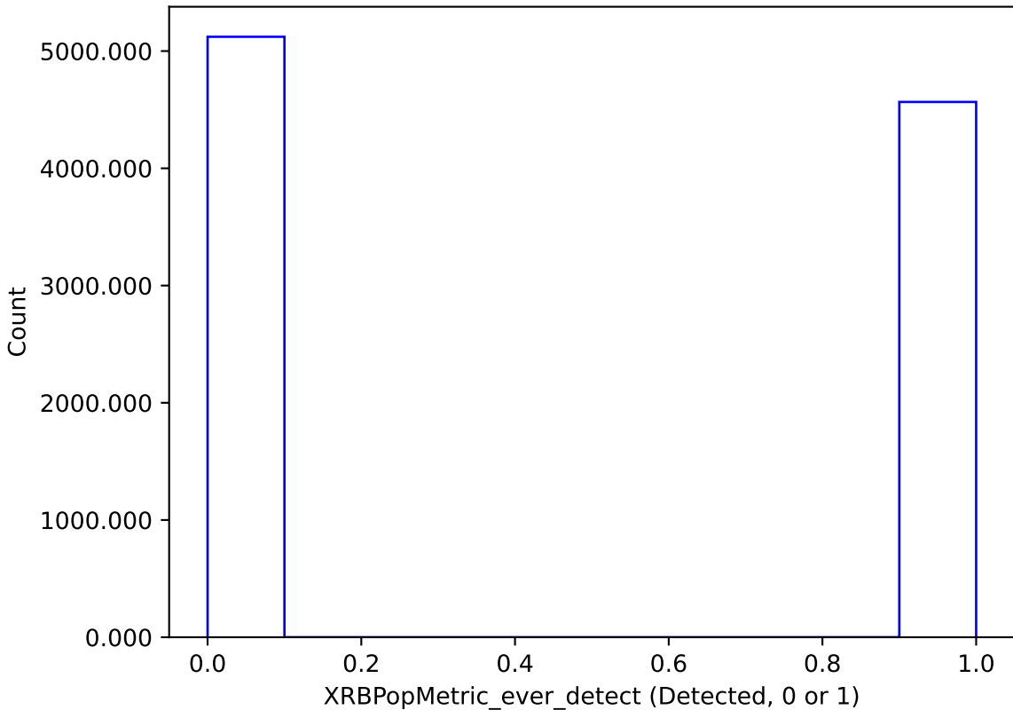
extra_ss_neo4_v3.4_10yrs : XRBPoMetric_ever_detect
