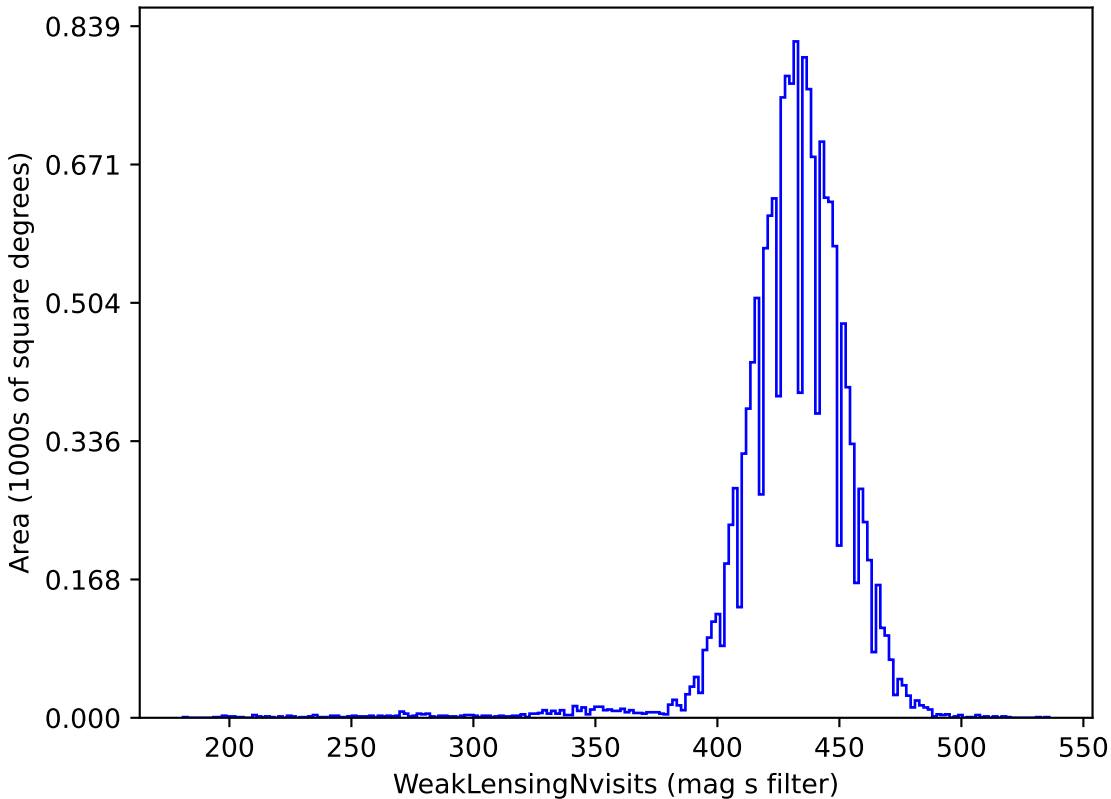
extra_ss_neo4_v3.4_10yrs gri band non-DD: WeakLensingNvisits
