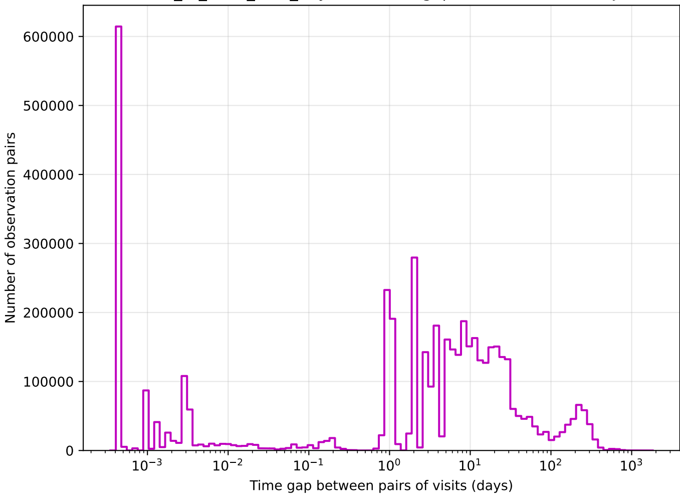
extra_ss_neo4_v3.4_10yrs z band: Tgaps observationStartMJD
