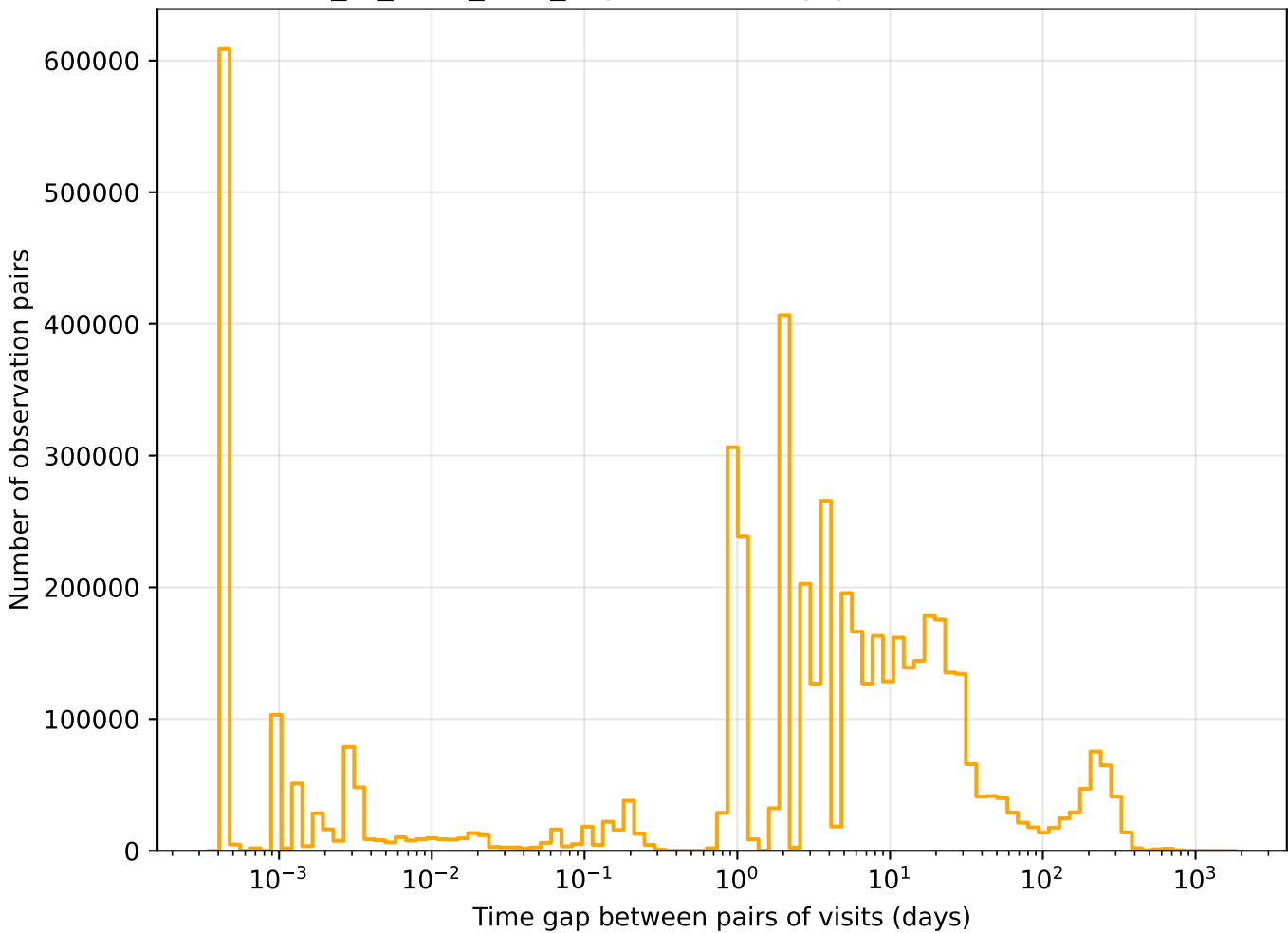
extra_ss_neo4_v3.4_10yrs r band: Tgaps observationStartMJD
