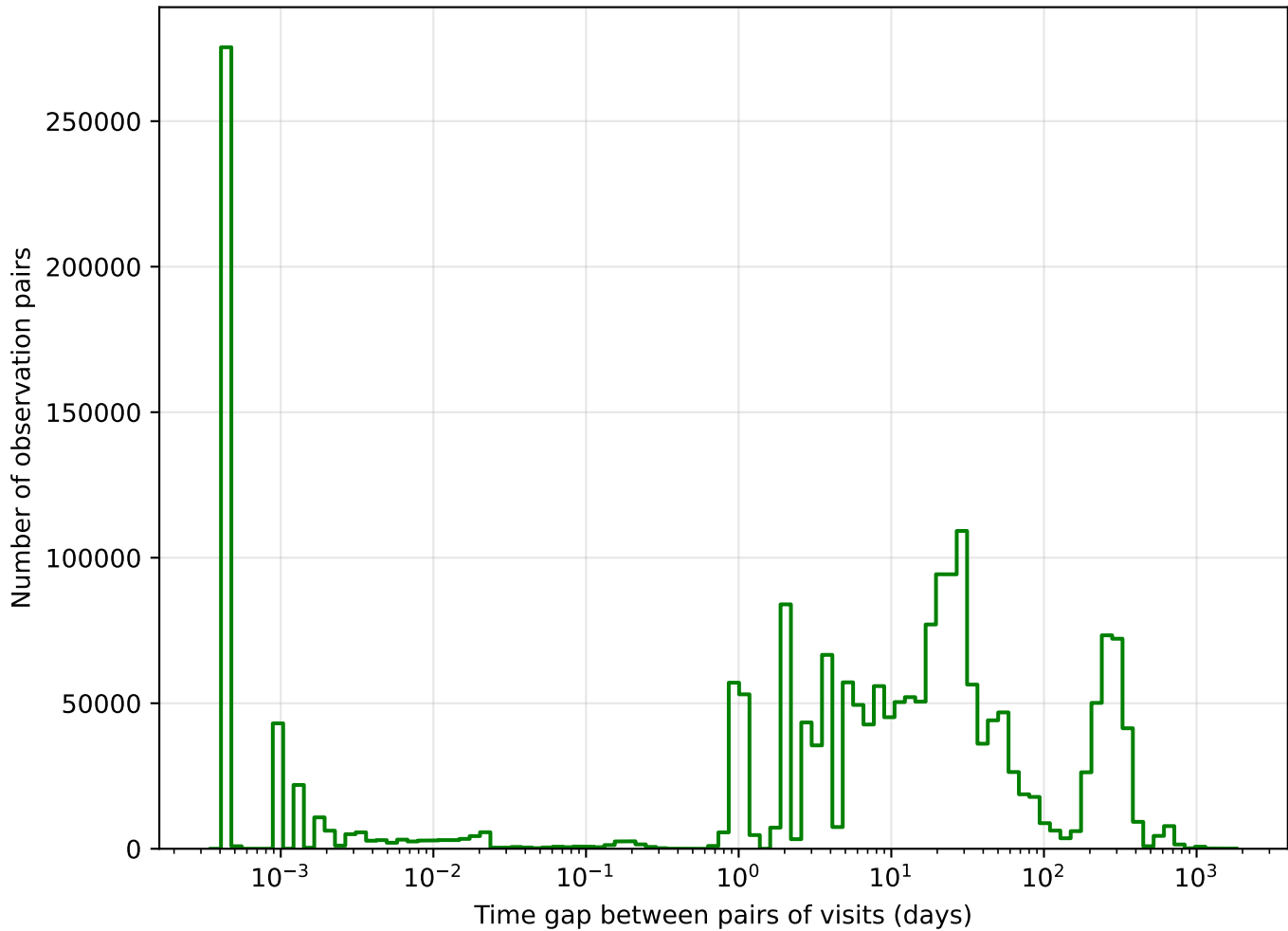
extra_ss_neo4_v3.4_10yrs g band: Tgaps observationStartMJD
