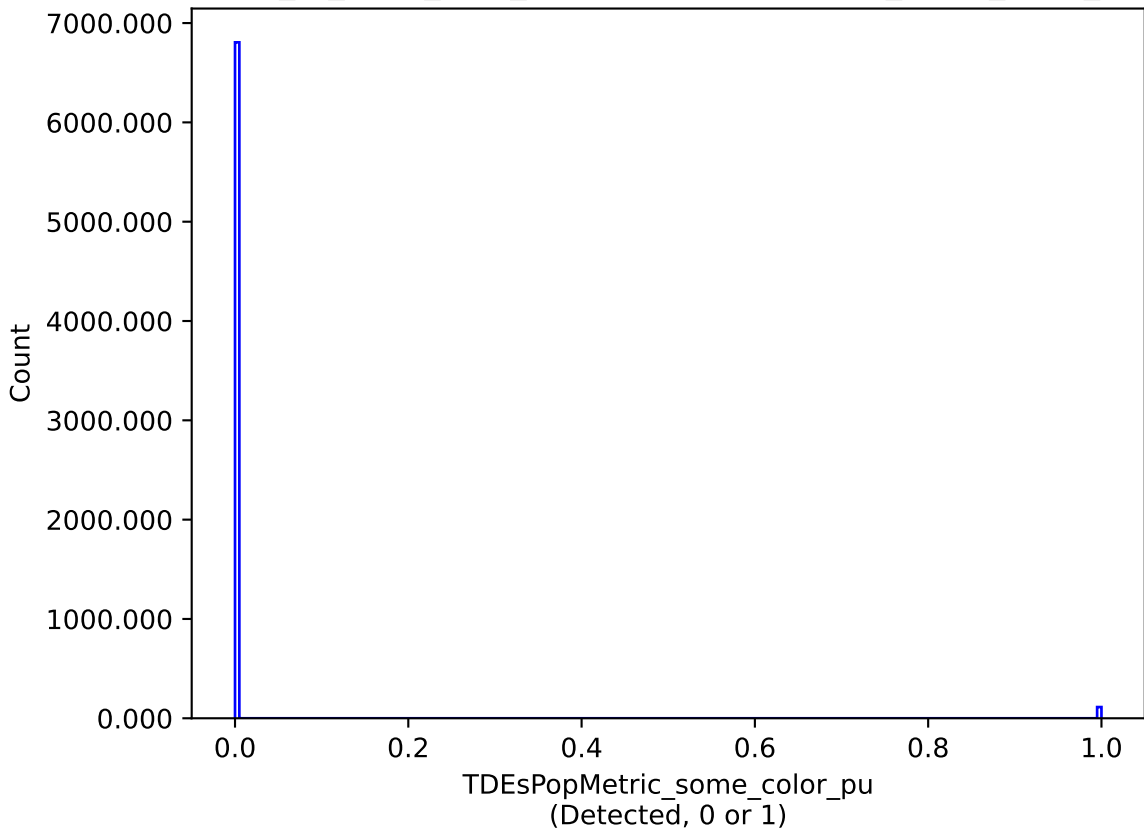
extra_ss_neo4_v3.4_10yrs : TDEsPopMetric_some_color_pu
