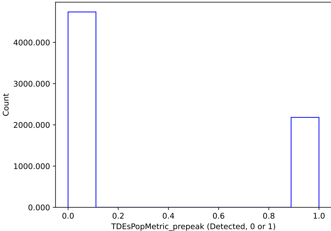
extra_ss_neo4_v3.4_10yrs : TDEsPopMetric_prepeak
