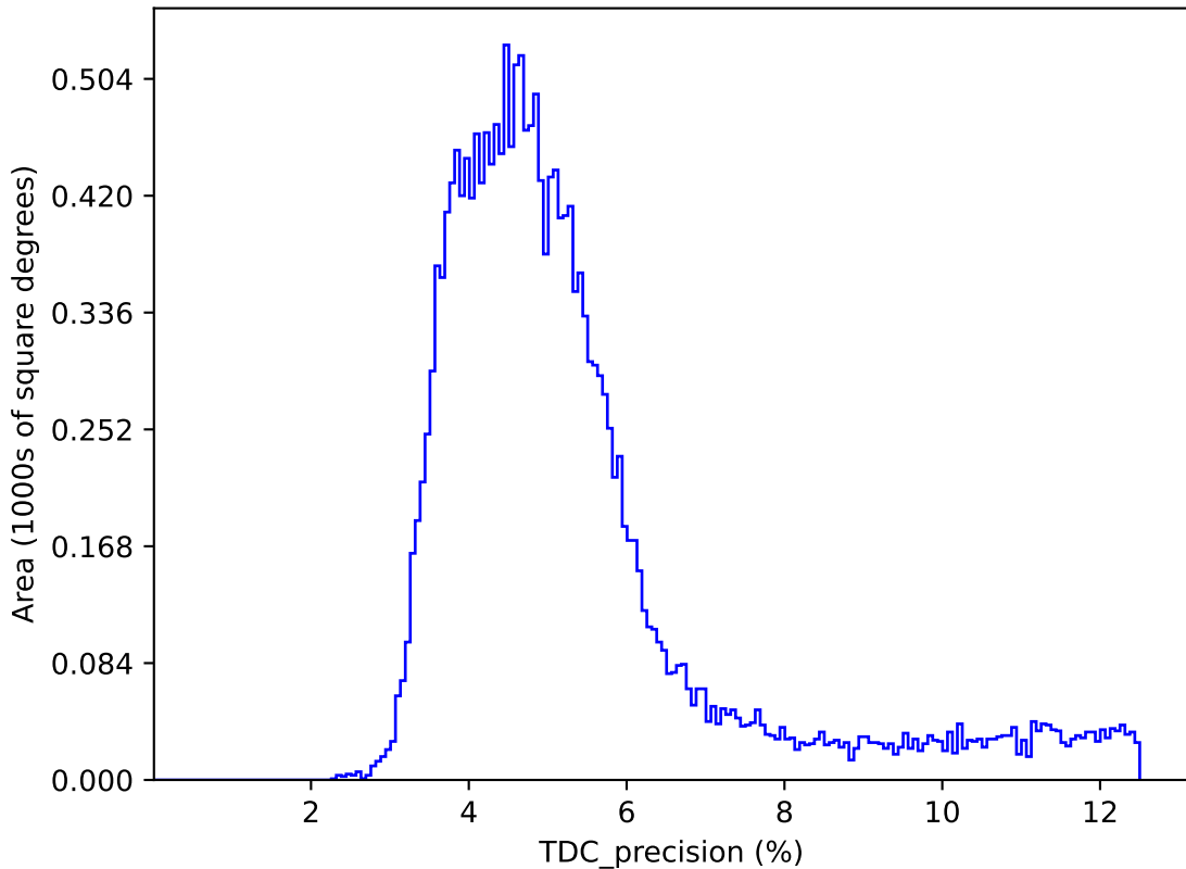
extra_ss_neo4_v3.4_10yrs : TDC_precision
